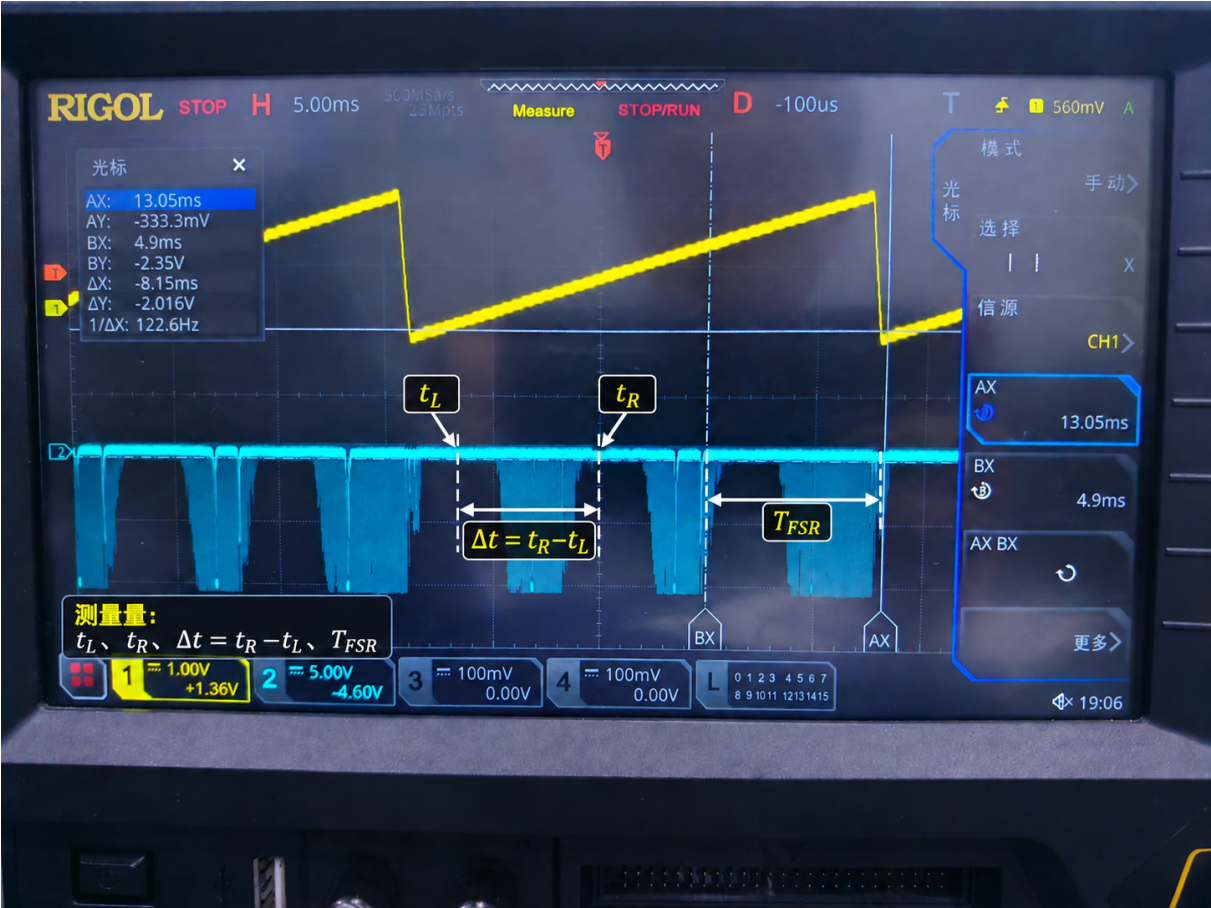
图 3 无限余辉下出光带宽测量的示波器记录及测量量标注。 Fig. 3 Oscilloscope record and measurement annotations for the output bandwidth under infinite persistence.
